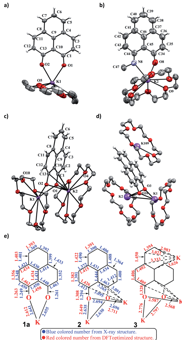
Fig. 1 (a) X-ray crystallographic structure of 1a(CE) . Ellipsoids are shown at 50% probability, selected bond lengths [ \text{\AA} ] and bond angles [deg]: K1–O1 2.6414, K1–O2 2.6551, O1–C1 1.2613, O2–C13 1.2490, O1–K1–O2 63.2271; (b) X-ray crystallographic structure of 1b(CE) . Ellipsoids are shown at 50% probability, selected bond lengths [ \text{\AA} ] and bond angles [deg]: K2–O8 2.5976, K2–N8 2.8418, O8–C34 1.2550, N8–C44 1.2939, O8–K2–N8 60.9823, K2–O8–C34 147.4870, K2–N8–C44 139.1102; (c) X-ray crystallographic structure of 2 . Ellipsoids are shown at 50% probability, selected bond lengths [ \text{\AA} ] and bond angles [deg]: K1–O1 2.6289, K1–O2 2.6350, O1–C1 1.2943, O2–C13 1.2955, K1–O1–K2 95.9253, K1–O2–K2 95.8503; (d) DFT optimized structure of 3 . A few selected bond lengths [ \text{\AA} ] and bond angles [deg]: K1–K2 4.0573, K1–O3–K2 97.7281; (e) bond distance analysis of 1a(CE) , 2 and 3 by X-ray structure and DFT study.
