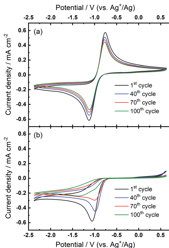
Fig. 1 (a) Cyclic voltammograms of the ORR and OER on an Au electrode at 100 \text{mV s}^{-1} in \text{O}_2 -saturated (a) 0.1 M \text{TBAClO}_4 /DMSO and (b) 0.1 M \text{Ca}(\text{ClO}_4)_2 /DMSO.
