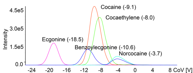
Fig. 4 Ionograms obtained during the CoV value ramp for cocaine and its metabolites infused at 100 ng mL –1 . The separation voltage was 2600 V and the modifier was acetonitrile.
