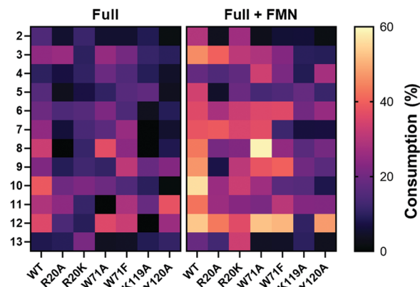
Fig. 7 Heat map of the consumption of compounds 2–13 by WT HiNfsB and its R20A, R20K, W71A, W71F, K119A and Y120A mutants. The reactions contained 2 mM substrate, 0.1 \mu M enzyme, 1 mM NADP + , 20 mM glucose, and 16 \mu M GDH in 100 mM phosphate buffer (pH 7.4) and were incubated at room temperature for 10 min. The data represent means \pm s.d. of three independent experiments.
