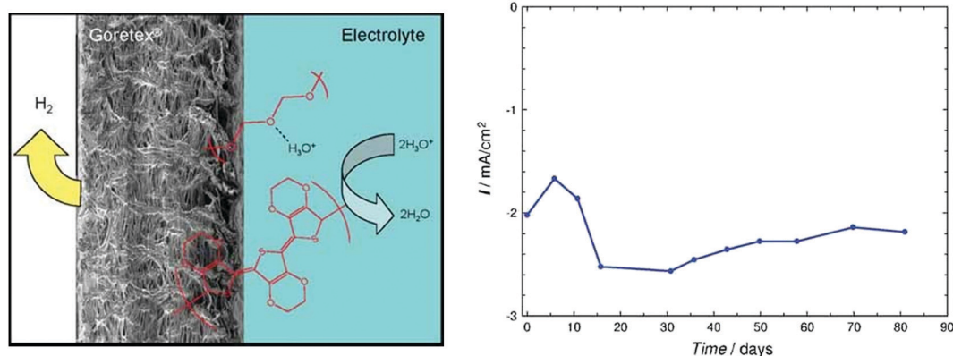
Fig. 94 Schematic of PEDOT-based HER electrode (left side). Long-term performance of PEDOT-PEG on Goretex/Au in 1 M H 2 SO 4 under N 2 at -0.35 V vs. SCE. Reproduced with permission from ref. 1339. Copyright 2010 Wiley.
