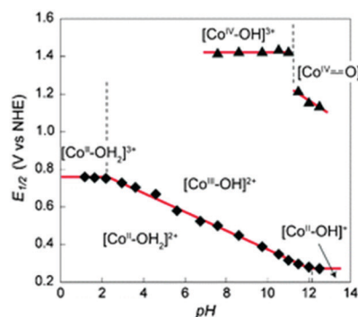
Fig. 130 A structural representation of [\text{Co}^{\text{II}}(\text{Py}5)(\text{OH}_2)](\text{ClO}_4)_2 (left image). Pourbaix diagram for [\text{Co}^{\text{II}}(\text{Py}5)(\text{OH}_2)](\text{ClO}_4)_2 . Reprinted with permission from ref. 1585 Copyright 2011 RSC.
