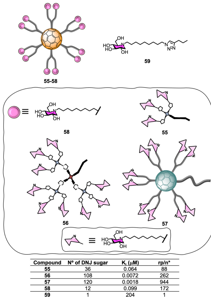
Fig. 13 General representation of glycofullerenes 55–58 and monovalent iminosugar 59 and their corresponding \alpha -Mannoside (JB \alpha -man) inhibitory activities ( K_i ). ^* \text{rp} = K_i (reference)/ K_i DNJ-fullerene, n = number of inhitope units relative to the inhitope number in the reference.
