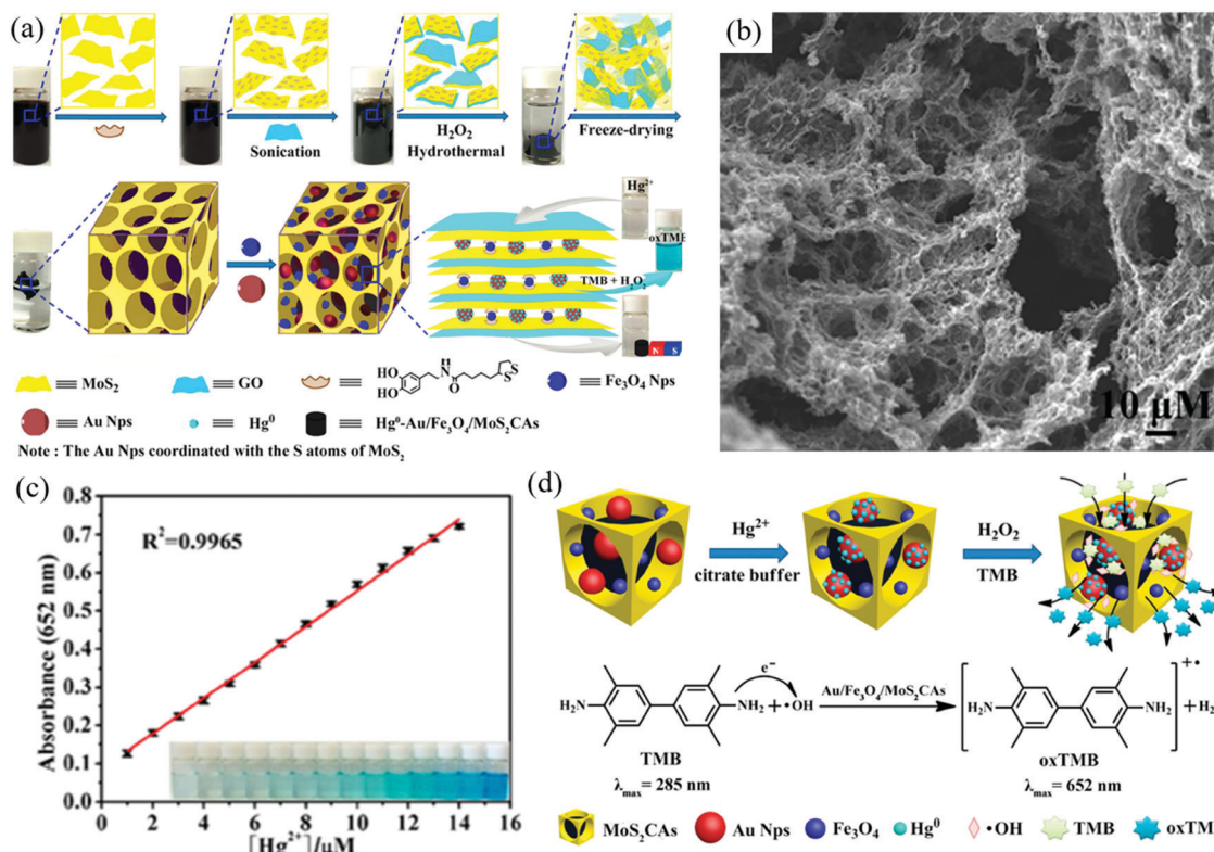
Fig. 4 Colorimetric detection of \text{Hg}^{2+} with 2DM aerogels: (a) The growth mechanism of \text{Au/Fe}_3\text{O}_4/\text{MoS}_2 CA. (b) The SEM diagram of \text{Au/Fe}_3\text{O}_4/\text{MoS}_2 CA. (c) The relationship between the absorption response of the detection system and the concentration of \text{Hg}^{2+} . (d) The detection mechanism of \text{Hg}^{2+} detection by \text{Au/Fe}_3\text{O}_4/\text{MoS}_2 CAs. 109 Copyright 2016, American Chemical Society.
