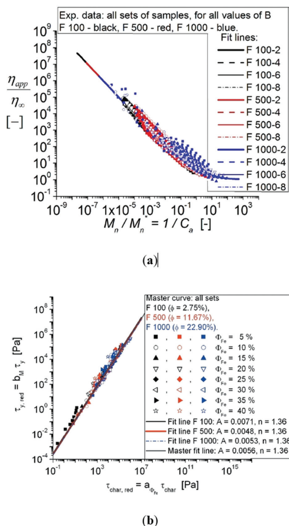
Fig. 38 Ferrofluid based MR fluids. (a) The dependence \eta_{app}/\eta_{\infty} = f(M_n/M_n^*) for different values of the Fe particle volume fraction \phi_{Fe} and of the magnetic nanoparticle volume fraction \phi . Fit lines: \eta_{app}/\eta_{\infty} = C_a + 2C_a^{1/2} + 1 . Fit parameter values are given in ref. 696; (b) master curve obtained for all samples with different nano and micro concentrations, at different values of magnetic field induction. a_{\phi} and b_M are horizontal and vertical translation coefficients of experimental data (reproduced from ref. 697 with permission from The Society of Rheology, copyright 2018).
