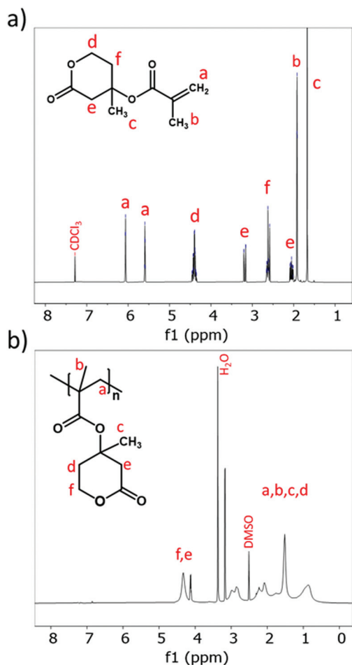
Fig. 1 ^1\text{H} -NMR spectra of MVLMA (a) and PMeVL (b).
