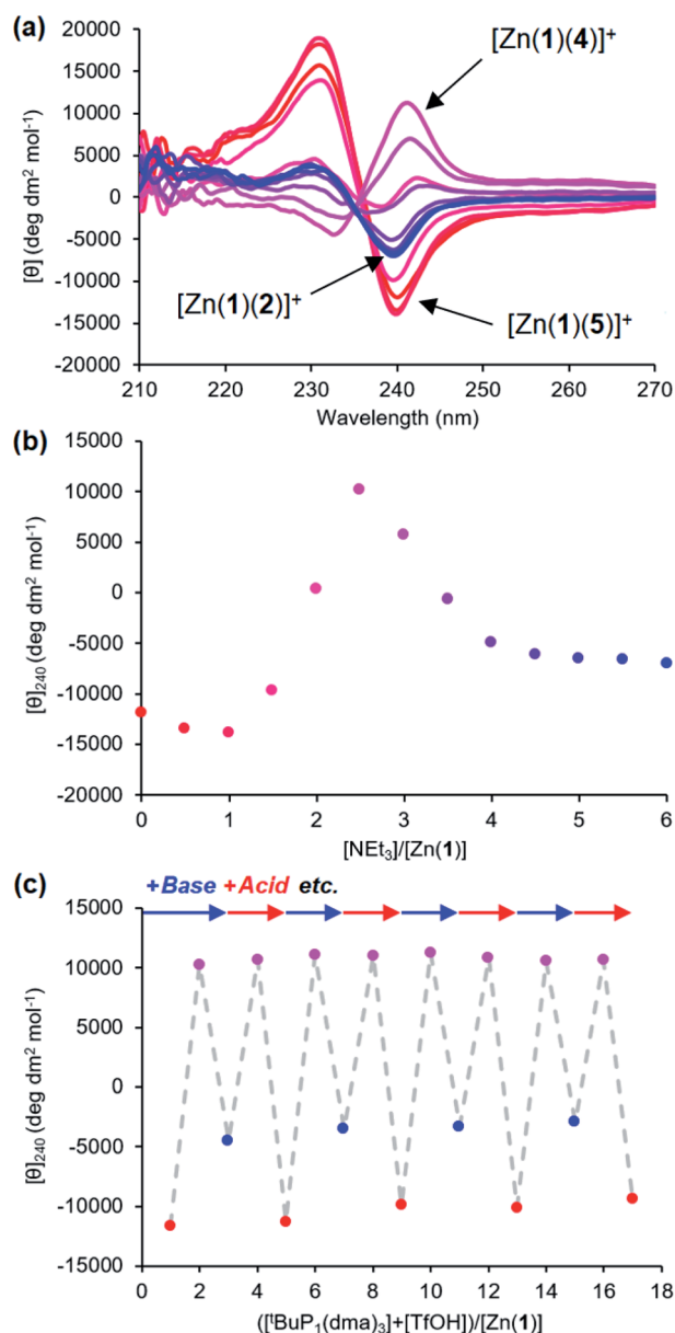
Fig. 9 (a) CD spectra of \text{Zn(1)} \cdot 2\text{ClO}_4 ( c_0 = 0.25 \text{ mM} ) with 2\text{-H} (1 eq.), 4\text{-H} (1 eq.) and 5\text{-H} (1 eq.) in MeCN with addition of \text{NEt}_3 (0.0 to 6.0 eq.) in 0.5 eq. increments; (b) molar ellipticity at 240 nm with addition of \text{NEt}_3 ; (c) molar ellipticity at 240 nm with alternating addition of ^t\text{BuP}_1(\text{dma})_3 ( \rightarrow ) and \text{TfOH} ( \rightarrow ) in 1 eq. increments.
