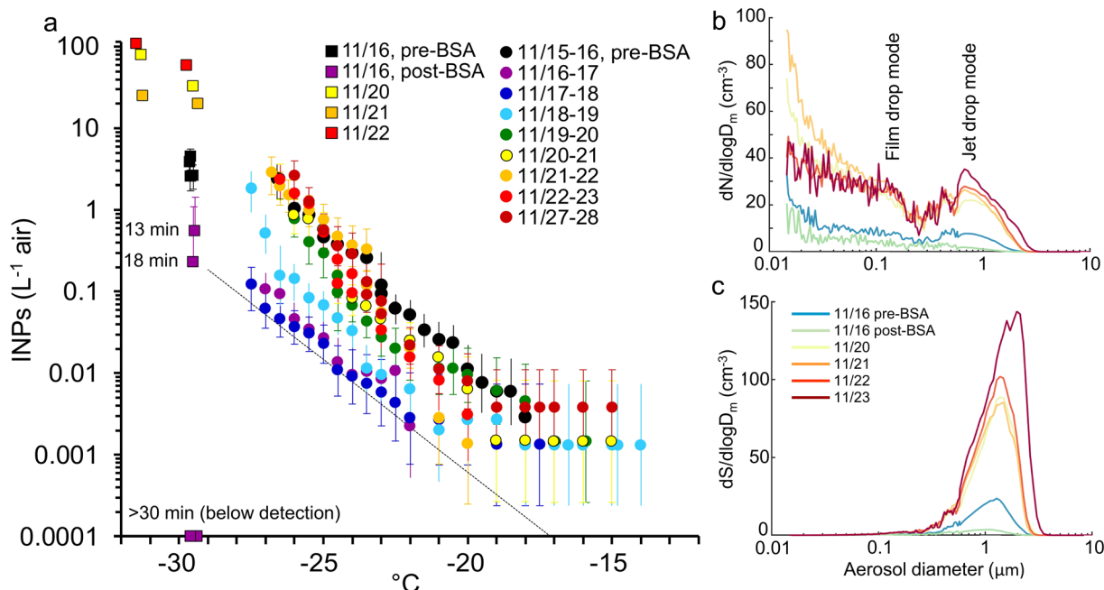
Fig. 5 a) INP spectra in the SSA measured with the ice spectrometer (circles) and the Continuous Flow Diffusion Chamber (squares) during the BSA + sugars addition experiment. The dashed line shows the estimated background INP level on filters. Numbers beside CFDC symbols show time after the addition of BSA + sugars. (b and c) aerosol emissions (dry) over the course of the experiment expressed on the basis of number and surface area, respectively. The post-BSA measures are the average of three scans taken 10–30 min after BSA addition.
