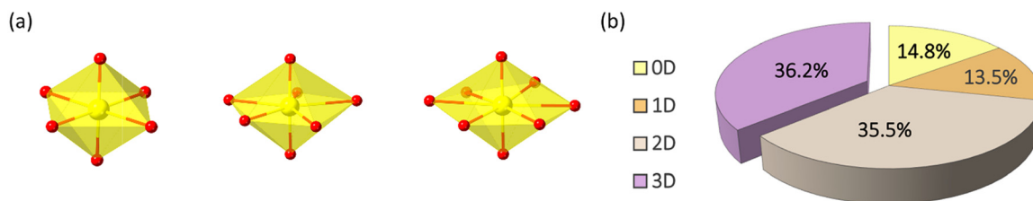
Fig. 1 (a) UO 6 , UO 7 , and UO 8 coordination polyhedrons in hexavalent uranyl phosphonates. (b) Distribution of 0D–3D uranyl phosphonate coordination polymers.
