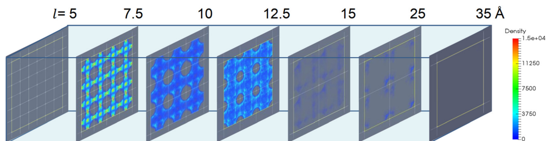
Fig. 10 The ethanol adsorption density distribution of W_s with fixed \sigma = 3 \text{ \AA} , \epsilon = 4.2 \text{ kJ mol}^{-1} for l = 5 \text{ \AA} ( 6 \times 6 \times 6 ), 7.5 \text{ \AA} ( 4 \times 4 \times 4 ), 10 \text{ \AA} ( 3 \times 3 \times 3 ), 12.5 \text{ \AA} ( 3 \times 3 \times 3 ), 15 \text{ \AA} ( 2 \times 2 \times 2 ), 25 \text{ \AA} ( 2 \times 2 \times 2 ) and 35 \text{ \AA} ( 1 \times 1 \times 1 ) structures.
