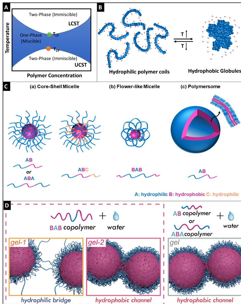
Fig. 3 Schematic representation of the phase diagram for the LCST and UCST thermo-responsive polymers (A), schematic diagram showing the phase transition of hydrophilic polymer coils ( < \text{LCST} ) to hydrophobic globule formation ( > \text{LCST} ), reproduced under Creative Commons license, 88 (B), a graphical illustration of self-assembly of amphiphilic block polymers (C), wherein core-shell micelle formation was observed for AB and ABA block copolymers (a), flower-like micelle formation was seen for the BAB block polymers and polymersome architecture was observed for AB polymers (c) reproduced under Creative Commons license, 88 and schematic diagrams of the gelling behavior of the BAB polymer through a hydrophilic bridge and hydrophobic channel for the BAB polymer (left side) and the gelling behavior of AB and ABA copolymers through hydrophobic channel formation (right side) based on the semi-bald model of micelles (D). Adapted with permission from ref. 114. Copyright © 2019, American Chemical Society.
