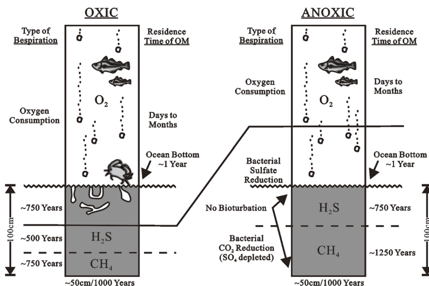
Fig. 4 The \text{O}_2 - \text{H}_2\text{S} - \text{CH}_4 level in oxic (left) and anoxic (right) depositional environments generally result in poor and good preservation of deposited organic matter, respectively. 71
