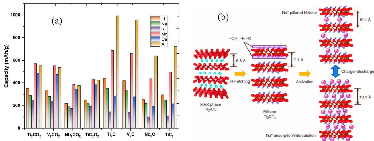
Fig. 21 (a) A study of the storage capacities of various MXene materials. (b) Diagram of the electrochemical activation in the Ti_2CT_x reaction mechanism, where MXene Ti_2CT_x was created by HF treatment from the precursor Ti_2AlC . The MXene Ti_2CT_x using expansion of Na^+ intercalation and reversible Na^+ (de)intercalation exhibits no alteration in interlayer distance. Reproduced from ref. 346 with permission from Springer Nature, copyright 2015.
