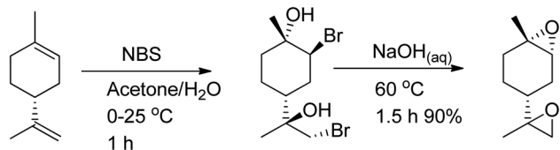
Scheme 26 Using both ( R )-(+)-limonene's exocyclic and endocyclic double bonds as starting materials, trans -LBE is synthesized via stereoselective di-bromohydration.
