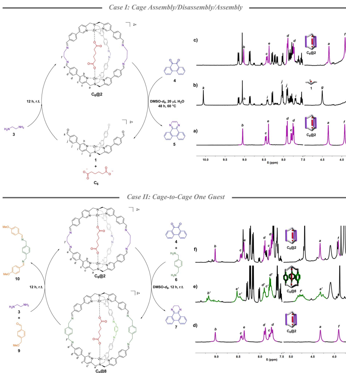
Fig. 1 Case I: partial 1 H-NMR (DMSO- d 6 , 400 MHz) of (a) C 6 @ 2 , (b) complex 1 obtained from the cage disassembly using quinone 4 , and (c) C 6 @ 2 re-formed after the addition of ethylenediamine 3 to the mixture. 1,3,5-Trimethoxy benzene is used as the internal standard. Case II: partial 1 H-NMR (DMSO- d 6 , 300 MHz) of (d) C 6 @ 2 , (e) C 6 @ 8 obtained after the addition of quinone 4 and p -xylenediamine 6 to C 6 @ 2 , and (f) C 6 @ 2 obtained after the addition of ethylenediamine 3 and p -anisaldehyde 9 to C 6 @ 8 . p -Xylene is used as the internal standard.
