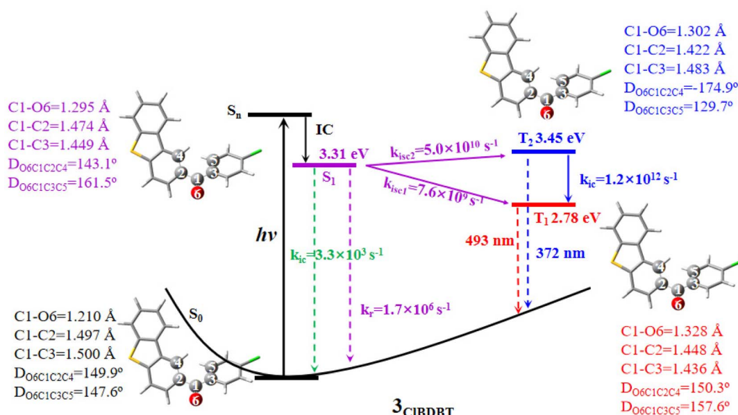
Fig. 3 The adiabatic energy levels, radiative ( k_r ) and nonradiative ( k_{ic} and k_{isc} ) rates, as well as T 1 and T 2 emission wavelengths for 3 CIBDBT . The ground state energy (−1660.75414666 a.u.) of 3 CIBDBT is set as the reference at the CC2/cc-pVDZ level. The geometrical parameters for some important bonds and dihedral angles are also shown.
