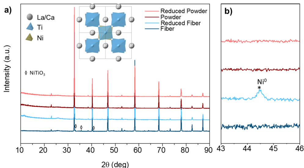
Fig. 1 Exsolution of Ni nanoparticles from LCNT perovskite materials. (a) XRD pattern of powder and fibers samples before and after reduced in 5% \text{H}_2/\text{N}_2 at 800 ^\circ\text{C} for 4 h. (b) The magnified 2\theta range between 43 to 46 ^\circ to illustrate the presence of Ni phase.
