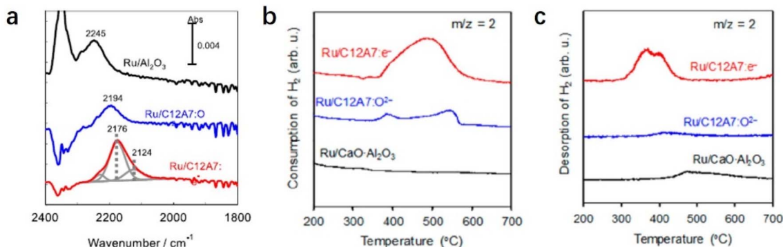
Fig. 6 (a) Difference FT-IR spectra of \text{N}_2 adsorbed on Ru/Al 2 O 3 , Ru/C12A7:O 2− , and Ru/C12A7:e − at -170 °C. Copyright 2012, Springer Nature. (b) \text{H}_2 -TPA and (c) Ar-TPD profiles of Ru/CaO·Al 2 O 3 , Ru/C12A7:O 2− , and Ru/C12A7:e − . Copyright 2015, Springer Nature.
