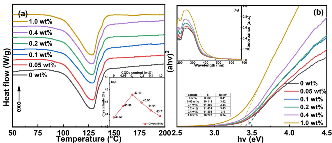
Fig. 6 (a) The DSC curves. (b) The Tauc plot. (a₁) The crystallinity. (b₁) The UV-vis absorption spectra of the samples with different CQD content.
