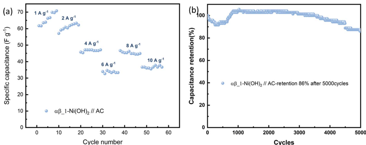
Fig. 11 (a) The specific capacitance evolution under various current densities of \alpha\beta_1 -Ni(OH) 2 //AC. (b) Cycling performance at 100 mA cm -1 for 5000 cycles.
