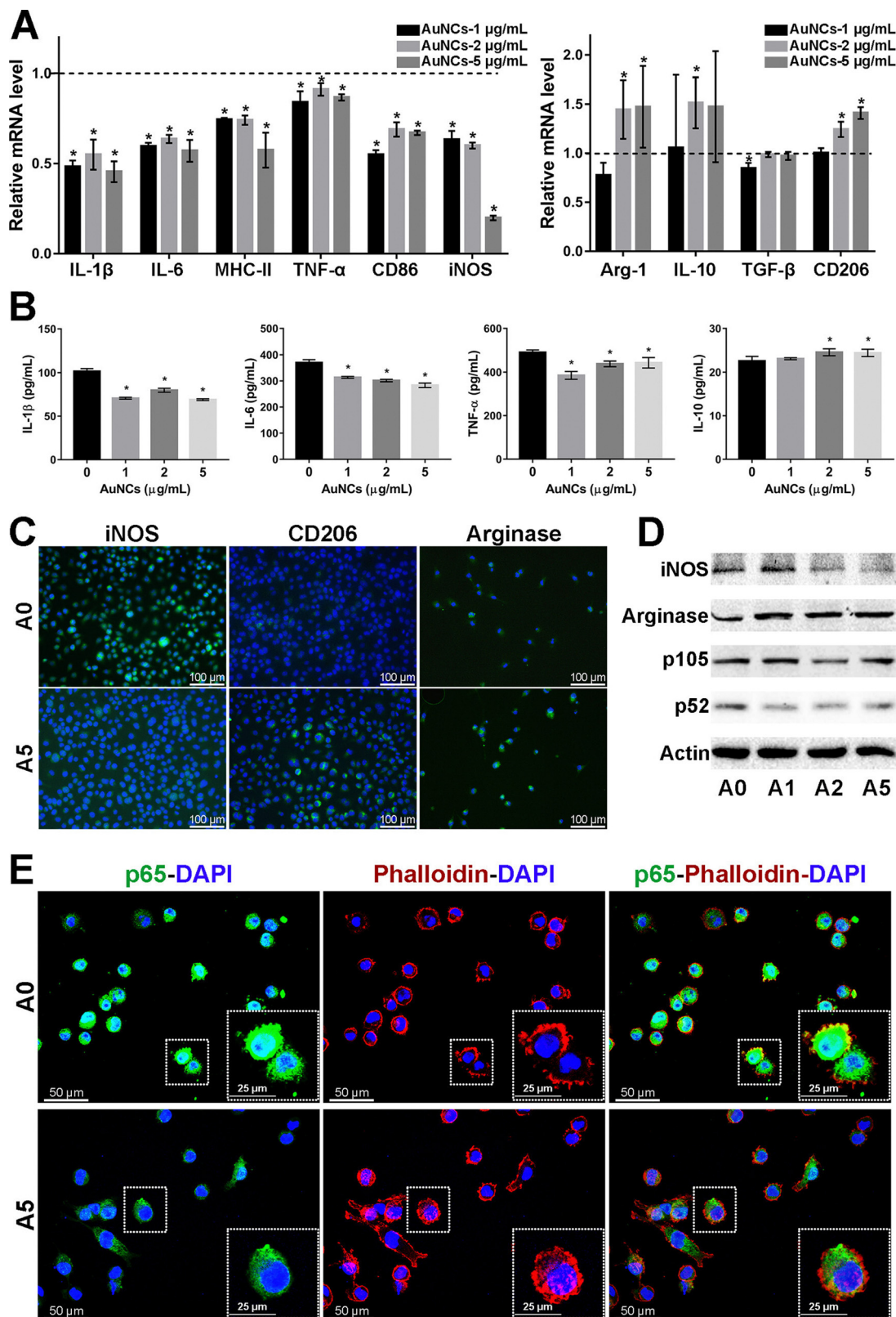
Fig. 2 Effect of AuNCs on the pro-inflammatory response of BV2 cells. (A) The represented mrna levels of AuNCs-1/2/5 \mu g mL ^{-1} groups were normalized to the control group and appeared as fold changes. (B) Quantification of cytokines in BV2 cell supernatant was performed by Elisa. (C) Represented if staining images of iNOS, CD206, and arginase (Alexa Fluor488, green) in BV2 cells. Nuclei were counterstained with dapi (blue). (D) Protein levels were examined by western blotting analysis. (E) The cell cytoskeleton was stained with phalloidin (bodipy 558/568, red). Nuclei were stained with dapi (blue). If staining of NF- \kappa B p65 (Alexa Fluor488, green) showed that in comparison with the control group, the cytoskeleton–nuclear translocation of p65 (original magnification, 400 \times ) was reduced in cells treated with AuNCs (5 \mu g mL ^{-1} ). Reprinted with permission from ref. 46. Copyright \copyright 2020, American Chemical Society.
