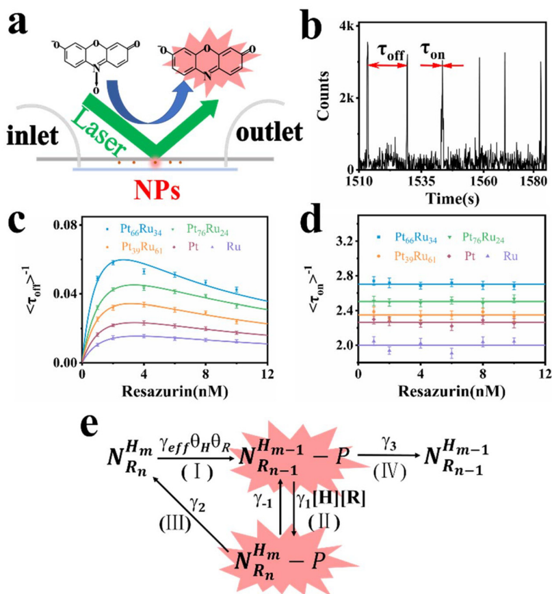
Fig. 2 (a) The experimental setup of fluorescent catalytic reactions based on TIRFM. (b) A segment of the fluorescence turnover trajectory of a \text{Pt}_{66}\text{Ru}_{34} nanocatalyst in saturated \text{H}_2 of 10 nM resazurin. (c) and (d) represent the tendency of the dependence of resazurin concentration on product formation rates and product desorption rates. Each data point is averaged over the turnover trajectories of more than 80 nanoparticles (NPs). (e) Kinetic mechanism of the reduction reaction. The meaning of each symbol is described in detail in the ESI†
