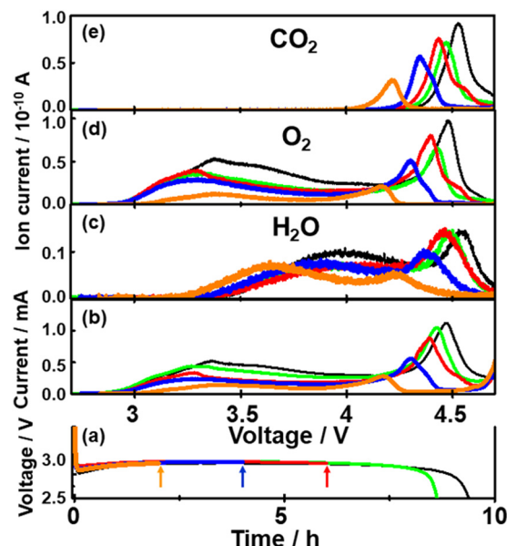
Fig. 7 (a) Discharge curves of various cells with discharge times of 2 (orange), 4 (blue), 6 (red), 8.8 (green), and 9.6 h (black). (b)–(e) Potential dependencies of (b) current and the background corrected ion currents of mass signals of (c) m/z = 18 ( H_2O ), (d) 32 ( O_2 ), and (e) 44 ( CO_2 ) as a function of time for 2 (orange), 4 (blue), 6 (red), 8.8 (green) and 9.6 h (black) discharged cells.
