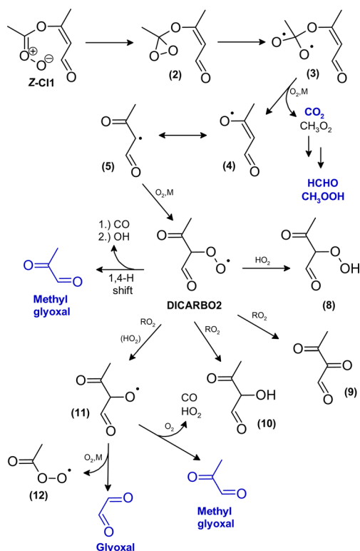
Scheme 2 Proposed mechanism for the fate of the carbonyl oxide Z-Cl1 yielding in fragmentation of the C 6 core structure. Species which were clearly identified as reaction products are marked in blue.
