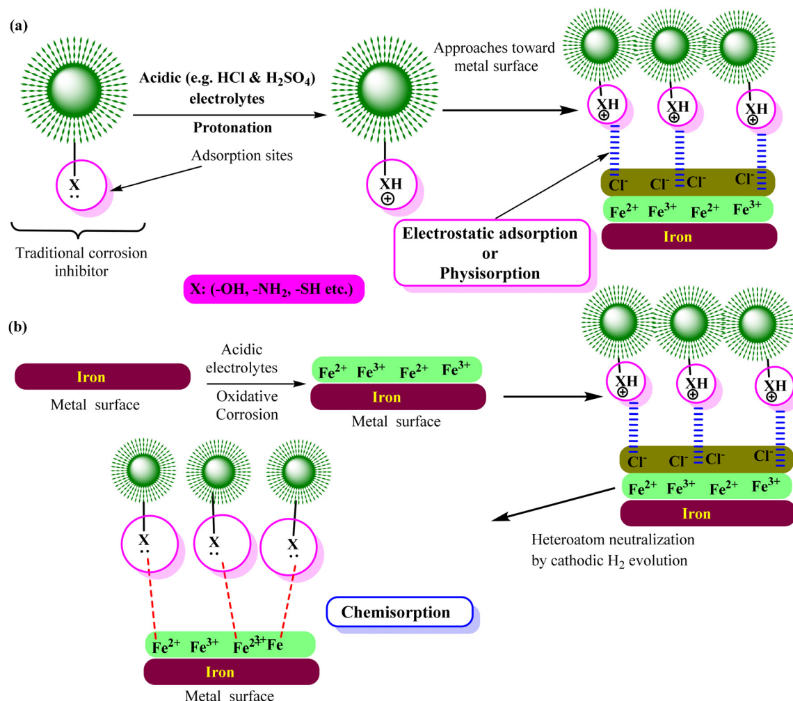
Fig. 5 Schematic presentation of the adsorption of a corrosion inhibitor having an amino ( -NH_2 ) substituent on steel surface in acidic ( HCl , H_2SO_4 , etc.) and the mode of physisorption and chemisorption [self-illustration, copyright permission not required].
