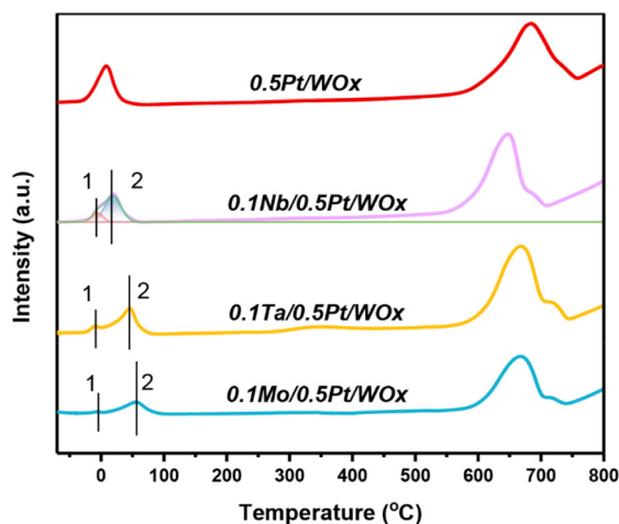
Fig. 3 \text{H}_2 -TPR profiles of 0.1M/0.5Pt/ \text{WO}_x catalysts.
