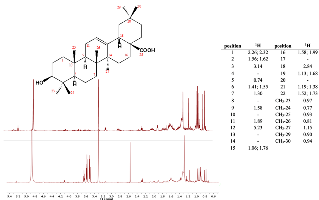
Fig. 1 Stereostucture of oleanolic acid and its chemical shifts in CD 3 OD; 1 H NMR spectrum of oleanolic acid (top) and of the extract in DMC of Aglianico grape pomace from Campania, Italy (bottom).
