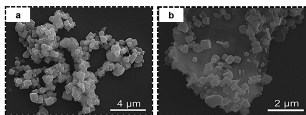
Fig. 26 SEM image of (a) Cs 2 AgBiI 6 showing agglomerated particles and (b) GO/Cs 2 AgBiI 6 showing less agglomerated particles. Reprinted with permission from ref. 138 Copyright 2023, Elsevier.
