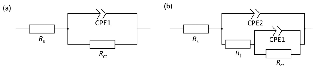
Fig. 3 EEC models used for EIS fitting. R_s , R_f and R_{ct} are the resistance of the solution, inhibitor/product film, and charge transfer, respectively. (a) \text{CPE1} is the constant phase element simulating the double layer capacitance, and (b) \text{CPE2} represents the response of inhibitor film/corrosion product film.
