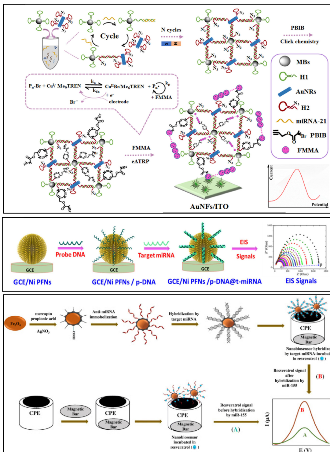
Fig. 9 (A) Two amplified sensors using SDA and eATRP for miRNA-21 detection, 127 (B) nickel phosphate flower-shaped nanostructure-modified GCE for miRNA detection, 128 and (C) core-shell Fe_3O_4@Ag nanoparticles for miRNA-155 detection. 129
