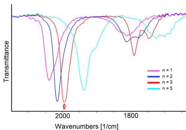
Fig. 6 Selected infrared spectra of [\text{Rh}_{12}\text{In}(\text{CO})_{28}]^{n-} as a function of the cluster charge n in \text{CH}_3\text{CN} containing 0.1 \text{ mol dm}^{-3} [\text{N}^n\text{Bu}_4][\text{PF}_6] . The absorptions of the solvent and supporting electrolyte have been subtracted. The red arrow indicates the initial spectrum.
