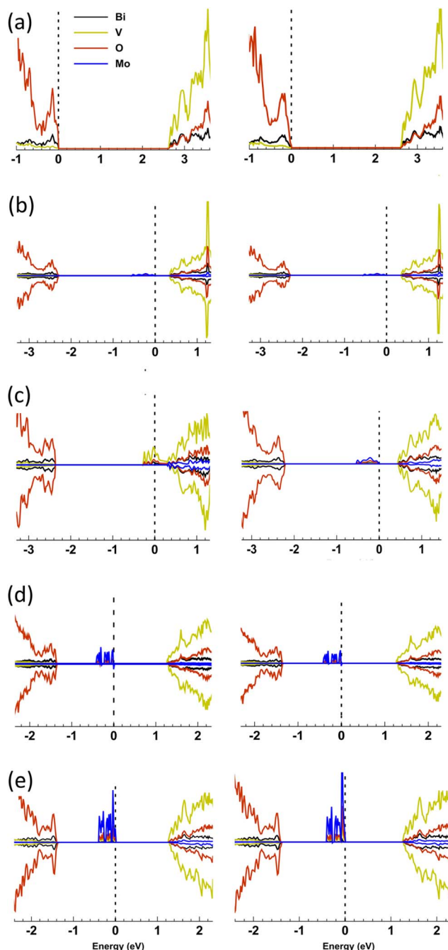
Fig. 11 Comparison of the PDOS for (left) t\text{-BiVO}_4 and (right) m\text{-BiVO}_4 host structures for (a) undoped, (b) 6.25 at% Mo in a V site, (c) 12.5 at% Mo in a V site, (d) 6.25 at% Mo in a Bi site, and (e) 12.5 at% Mo in a Bi site. For each host structure, the VBM, formed primarily by O orbitals, are plot at the same position to one another. The PDOS are drawn for energies \sim 1 eV below the VBM up to \sim 1 eV above the CBM, which is formed primarily by V orbitals. The dashed line represents the highest occupied state in each structure.
