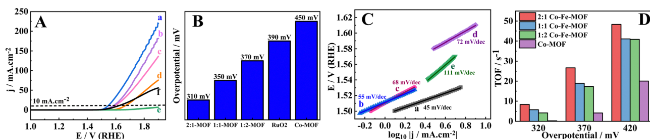
Fig. 5 LSV polarization curves (A) of MOFs measured at a scan rate of 5 \text{ mV s}^{-1} in 1.0 M KOH at a rotation rate of 1600 rpm for (a) \text{GC}_{\text{RDE}}/2:1 \text{ Co-Fe-MOF} , (b) \text{GC}_{\text{RDE}}/1:1 \text{ Co-Fe-MOF} , (c) \text{GC}_{\text{RDE}}/1:2 \text{ Co-Fe-MOF} , (d) \text{GC}_{\text{RDE}}/\text{Co-MOF} , (e) \text{GC}_{\text{RDE}}/\text{Fe-MOF} , and (f) \text{GC}_{\text{RDE}}/\text{RuO}_2 ; the corresponding bar diagrams (B) depicting the overpotentials at 10 \text{ mA cm}^{-2} ; (C) Tafel slopes of (a) \text{GC}_{\text{RDE}}/2:1 \text{ Co-Fe-MOF} , (b) \text{GC}_{\text{RDE}}/1:1 \text{ Co-Fe-MOF} , (c) \text{GC}_{\text{RDE}}/1:2 \text{ Co-Fe-MOF} , (d) \text{GC}_{\text{RDE}}/\text{Co-MOF} , and (e) \text{GC}_{\text{RDE}}/\text{RuO}_2 ; and (D) TOF plots of MOFs at different overpotentials.
