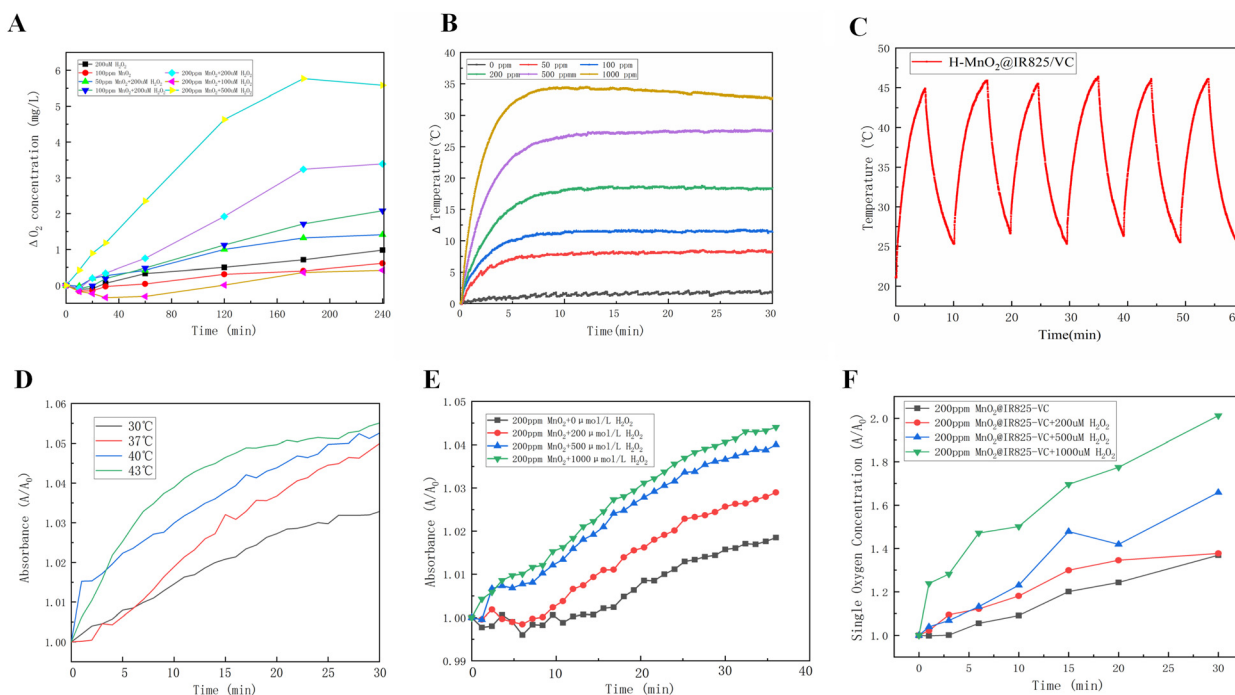
Fig. 2 Examination of the performance characteristics of the nanoparticles. (A) Curves showing the oxygen concentration with respect to time in an H-MnO 2 solution (200 ppm) containing H 2 O 2 at concentrations of 0, 200, 500, and 1000 μM. (B) Curves of the temperature change with respect to time for an H-MnO 2 @IR825-VC solution subjected to laser irradiation. The concentration of H-MnO 2 @IR825-VC was set to 0, 50, 100, 200 and 500 ppm. (C) Verification of the photothermal stability of H-MnO 2 @IR825-VC. The curve shows the change in the temperature of the H-MnO 2 @IR825-VC solution with time by turning the laser switch on or off every 5 min, with 10 min as one cycle. (D) Time-course absorbance curves showing the amount of hydroxyl radicals produced by the reaction of H-MnO 2 @IR825-VC (200 ppm) and H 2 O 2 (500 μM) at a pH level of 5.0 and varying temperatures: 30, 37, 40 and 43 °C. (E) Time-course absorbance curves showing the amount of hydroxyl radicals produced by the reaction of H-MnO 2 @IR825-VC (200 ppm) containing H 2 O 2 at concentrations of 0, 200, 500, and 1000 μM. (F) When exposed to laser irradiation, time-course absorbance curves showing singlet oxygen produced by the reaction of H-MnO 2 @IR825-VC (200 ppm) containing H 2 O 2 at concentrations of 0, 200, 500, and 1000 μM.
