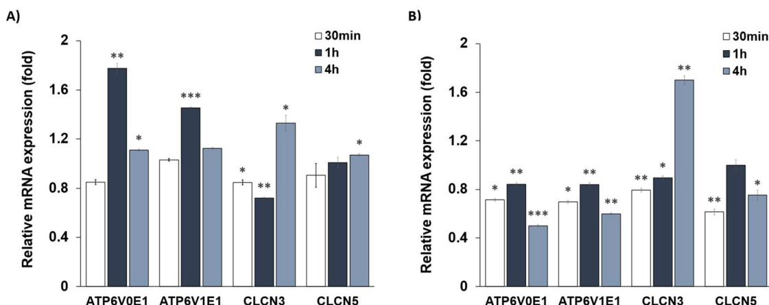
Fig. 5 Endosome escape related gene expression levels at (A) 330 and (B) 500 mOsm \text{kg}^{-1} osmolality at various incubation times. Gene expression levels at 330 and 500 mOsm \text{kg}^{-1} osmolality were normalized by those at 280 mOsm \text{kg}^{-1} osmolality. The results are expressed as mean \pm SE ( n = 3 ). Statistical differences are indicated as *: p < 0.05 , **: p < 0.01 , and ***: p < 0.001 .
