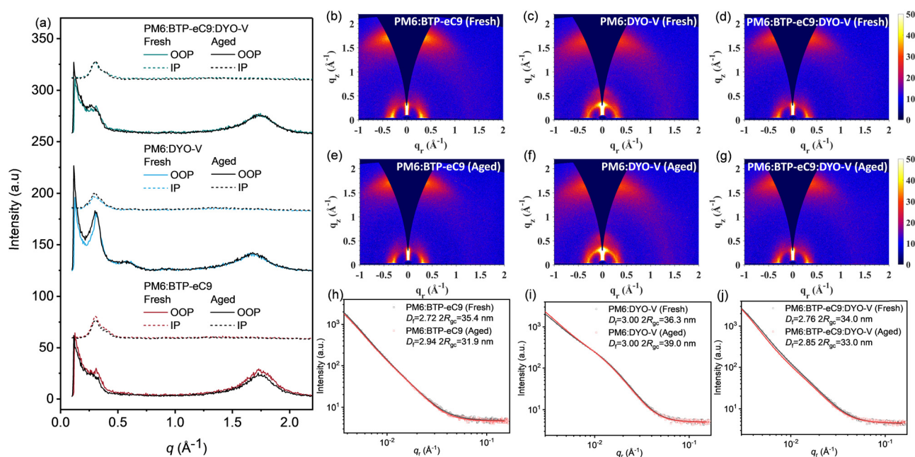
Fig. 4 (a) 1-D GIWAXS line-cuts along the in-plane (IP) and out-of-plane (OOP) directions for fresh and aged blend films. 2D GIWAXS plots of the PM6:BTP-eC9, PM6:DY0-V and PM6:BTP-eC9:DY0-V (b)–(d) fresh and (e)–(g) aged samples. (h)–(j) Corresponding in-plane GISAXS line-cuts of the fresh and aged blend films.
