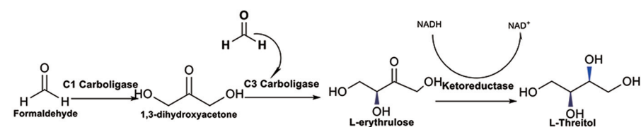
Scheme 1 Representative examples of threitol synthesis. 9–13
