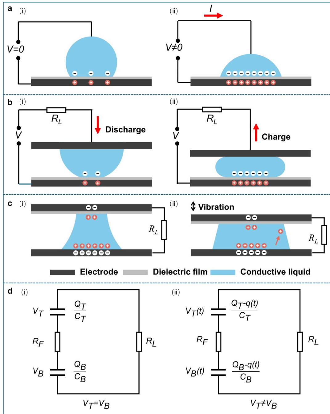
Figure 3. Basic working principles and equivalent circuit diagram. a) Working principle of the EWOD process. (i) no external voltage applied between the metal and the electrolyte solution, (ii) external voltage applied between the metal and the electrolyte solution. b) Working principle of the REWOD process. c) Working principle of the water bridge REWOD process. d) Equivalent circuit diagram of the water bridge REWOD process.
