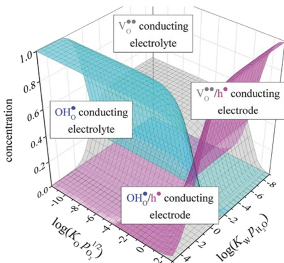
Fig. 7 The concentration of holes, oxygen ions and hydroxyl groups in perovskite oxides as a function of water partial pressure ( P_{H_2O} ), oxygen partial pressure ( P_{O_2} ) and equilibrium constants of hydration reaction ( K_W ) and oxygenation reaction ( K_O ). This figure has been adapted from ref. 122 with permission from John Wiley & Sons, copyright 2025.
