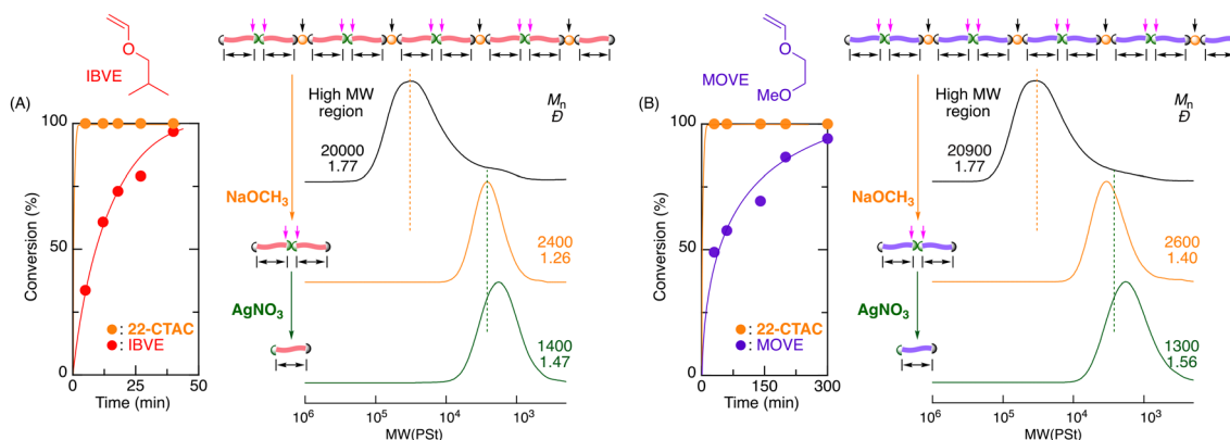
Fig. 8 Cationic DT copolymerization of IBVE (A) and MOVE (B) with 22-CTAC and SEC curves before and after stepwise degradation: [VE]_0/[22-CTAC]_0/[I]_0/[ZnCl_2]_0 = 4000/200/20/4.0 mM in CH_2Cl_2/n -hexane/ Et_2O (20/10/10) at -40 °C. [Thioacetal\ unit]_0/[AgNO_3]_0 = 5.0/50 mM in THF/ H_2O at 20 °C. [Carbonate]_0/[NaOCH_3]_0 = 5.0/50 mM in CH_3OH at 60 °C.
