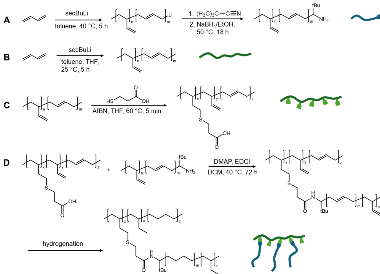
Fig. 1 Reaction scheme of (A) amine-terminated 1,4-PB, n/(m+n) = 0.12 ; (B) 1,2-PB, n/(m+n) = 0.89 ; (C) carboxyl functionalized 1,2-PB, and (D) polyethylethylene-graft-polyethylene.
