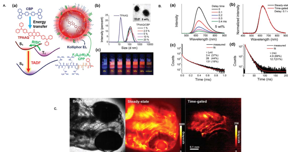
Fig. 24 (A) (a) Representation of TPAAQ/CBP/CPA TADF nanoparticles (b) DLS histograms showing the size of the nanoparticles and inset TEM images showing their morphology. (c) Photographs of the nanoparticle solutions under UV irradiation. (B) Time-gated emission spectra of the nanoparticles at various delay times. (C) Imaging of zebrafish incubated with TPAAQ/CBP/CPA nanoparticles, where the bright field is displayed on the left side of the figure, the steady-state luminescence is shown in the middle, and the time-gated luminescence is displayed on the right. Reproduced from ref. 173 with permission from John Wiley & Sons, Copyright © 2024, Wiley-VCH Verlag GmbH & Co. KGaA, Weinheim.
