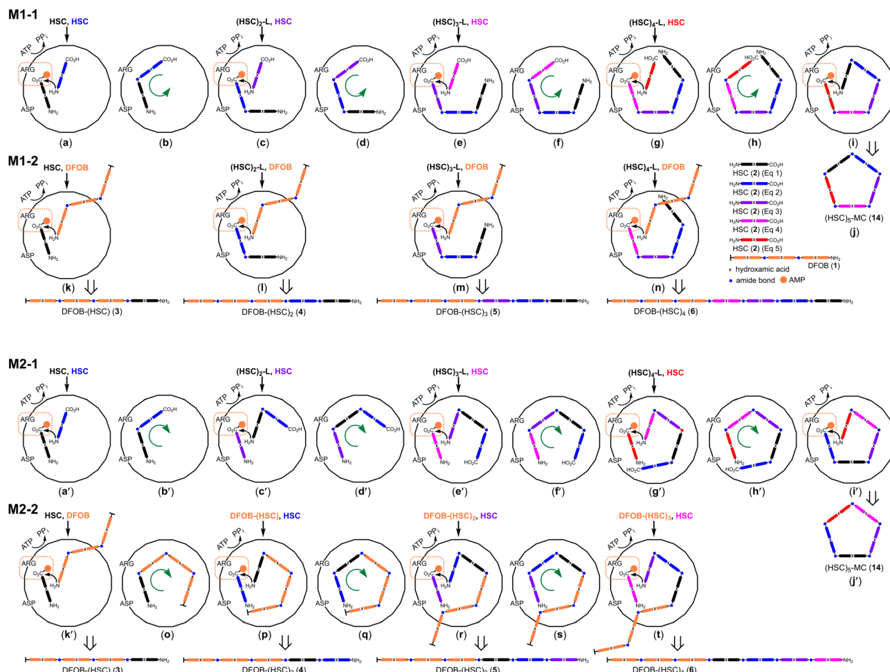
Scheme 3 Putative StDesD-mediated assembly of macrocyclic (HSC) 5 -MC (14) by a processive mechanism with 2 predominating as the nucleophilic (M1-1: (a–i)) or carboxylate-activated (M2-1: (a'–i')) substrate. Putative assembly of DFOB-(HSC) x ( x = 1–4 ) (3–6, respectively) with 1 conserved as the nucleophilic substrate for condensation with pre-assembled carboxylate-activated 2 or 2 oligomers (M1-2: (k–n)), or 2 conserved as the carboxylate-activated substrate for condensation with 1 or 3–5 as pre-assembled nucleophilic substrates (M2-2: (k'–t)). Intra-cavity procession of intermediate substrates (green arrow) would enable the position of the carboxylic acid group of 2 or 2 oligomers is conserved for activation (broken orange box).
