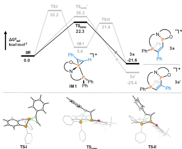
Fig. 4 Computed mechanism at the PW6B95-D4/def2-QZVPP(SMD: CH_2Cl_2 )/ r^2 -SCAN-3c(CPCM: CH_2Cl_2 ) level of theory for the addition of phenylacetylene to 2a (black), as well as other higher energy pathways (grey) and transition state structures.
