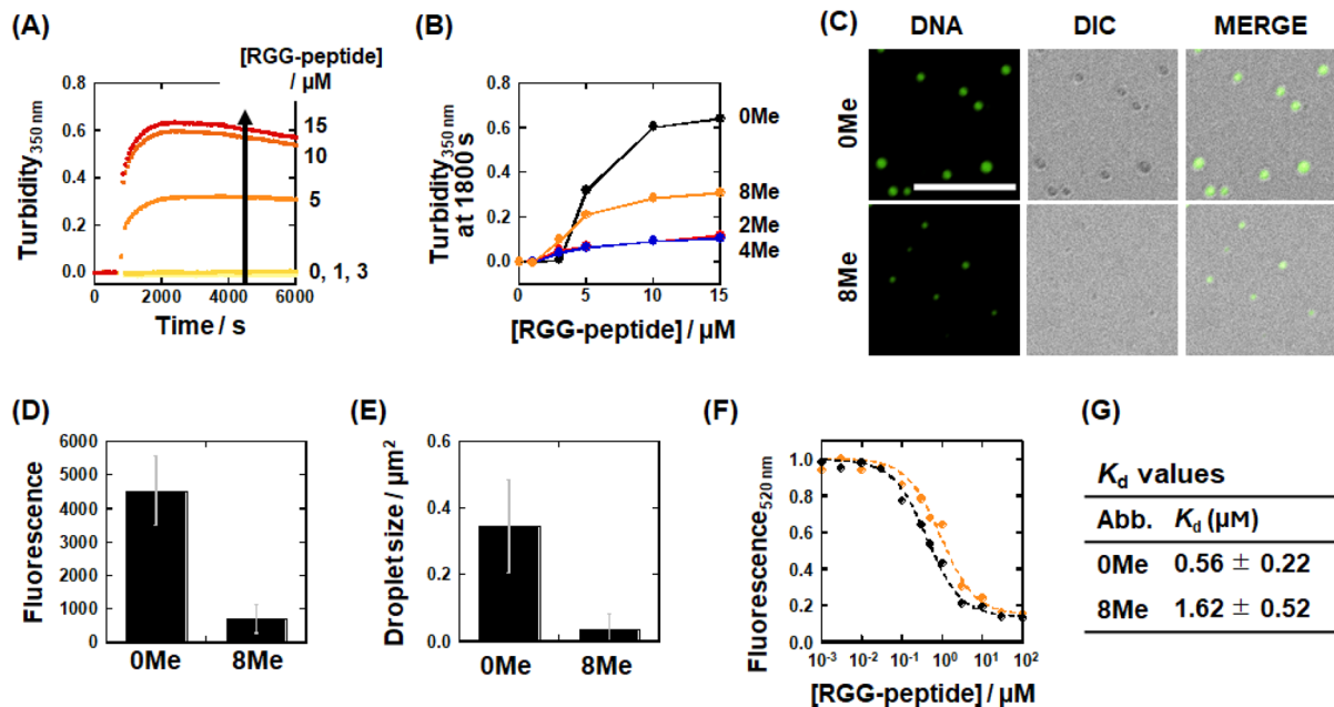
Fig. 1 (A) Turbidity changes at 350 nm for a mixture of 5 μM 0Me DNA and various concentrations of RGG-peptide (0, 1, 3, 5, 10, and 15 μM) in a buffer containing 100 mM KCl, 1 mM K_2EDTA , and 10 mM K_2HPO_4 (pH 7.0) at 25 °C. Note that data with 0, 1, and 3 μM RGG-peptide are overlapped. (B) Turbidity 350nm at 1800 s for 5 μM DNAs with differing methylation levels (black; 0Me, red; 2Me, blue; 4Me, orange; 8Me) against various RGG-peptide concentrations (0, 1, 3, 5, 10, and 15 μM). (C) Fluorescence microscopy images showing the mixture of 5 μM FAM-labeled DNAs with 5 μM RGG-peptide after incubation for 1800 s. Scale bar = 10 μm (D) bar graph showing total fluorescence intensity from inside of droplets for 0Me and 8Me with RGG-peptide. (E) Average droplet size for 0Me and 8Me. (F) Plots of relative fluorescence intensity at 520 nm for 50 nM FAM-0Me (black) and FAM-8Me (orange) as a function of RGG-peptide concentration. All measurements were carried out in the KCl buffer at 25 °C. (G) Dissociation constant ( K_d ) values for 0Me and 8Me with RGG-peptide in the KCl buffer at 25 °C.
