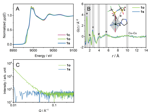
Fig. 2 (A) XANES profiles. (B) PDF analysis. G(r) is plotted to radius. Inset schematic representation indicates the dominantly corresponding distance correlations. (C) SAXS profiles. \text{CuK}\alpha X-ray source was used.
