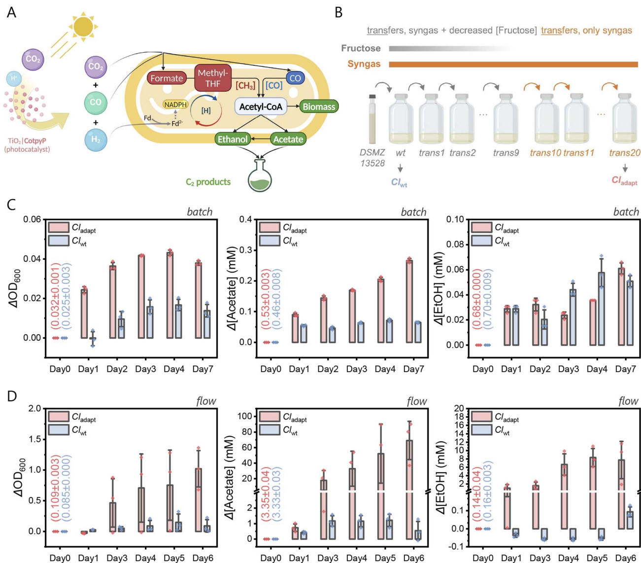
Fig. 1 Adaptive laboratory evolution (ALE) of C. ljungdahliae . (A) Schematic illustration of the syngas-fermenting metabolic pathways in C. ljungdahliae ( C_l ), including integration with photocatalytic syngas production. [\text{CH}_3] (red color), methyl branch; [\text{CO}] (blue color), carbonyl branch. (B) Schematic summary of the ALE process. The wild-type strain ( C_{l_{\text{wt}}} ) was adapted to a syngas environment through gradual fructose reduction and removal over 20 transfers, resulting in the adapted strain ( C_{l_{\text{adapt}}} ). (C) Comparative analysis of growth and \text{C}_2 product generation (acetate and ethanol) between C_{l_{\text{adapt}}} and C_{l_{\text{wt}}} under batch gas purging conditions (syngas purging for 30 min daily, 112 mL headspace). (D) Similar comparative analysis under continuous gas flow conditions (10 mL syngas per min). Growth conditions: ATCC Medium 1754 (pH 5.9), 37 °C with 150 rpm mixing. Numbers in brackets indicate the values at the start of the experiment.
